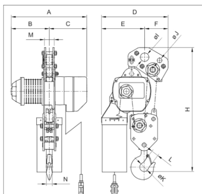
575 SERIES
