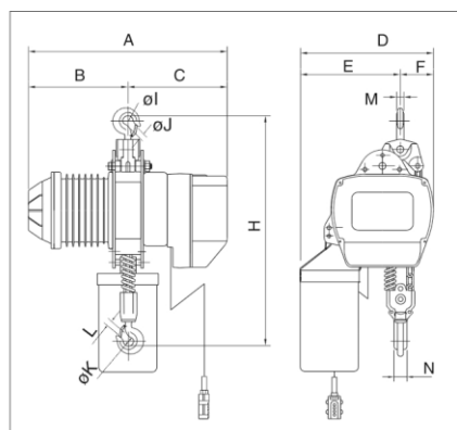
520~550 SERIES
