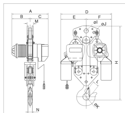
5100 SERIES
